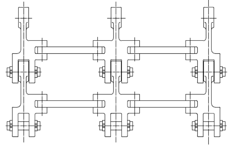
Triple Link
